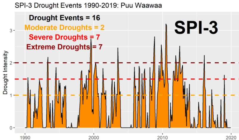
Figure 12. 30-year (1990-2019) SPI-3 time series (reversed axis) at Pu'u Wa'awa'a.
