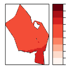
StDs ANN RCP 8.5 (5.8 °F)
