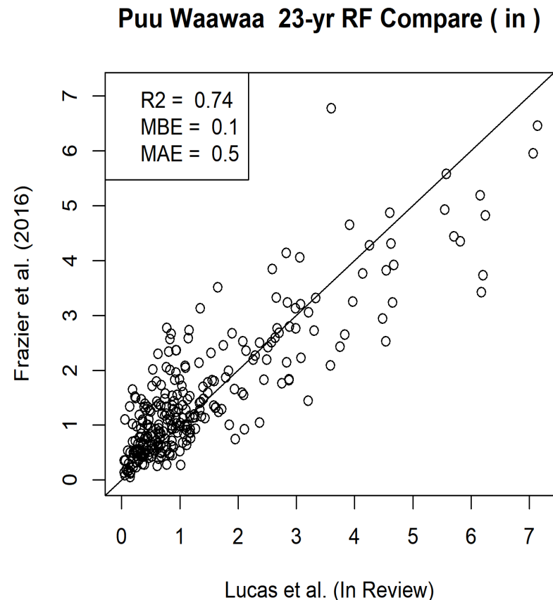
Figure A1: One to one comparison of 23-years (1990-2012) of monthly rainfall from two unique datasets for Pu'u Wa'awa'a, and associated error metrics; R2, is the coefficient of determination, MBE, is the mean bias error, MAE, mean absolute error.
