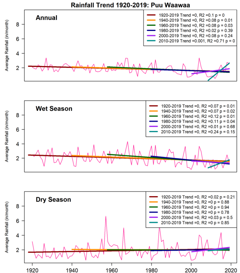
Figure 9. 100-year (1920-2019) rainfall time series at Pu'u Wa'awa'a with linear trends calculated over six unique periods in the record; Trend is the slope (inches per year); R2 is the strength of the trend; p is a measure of the statistical significance.
