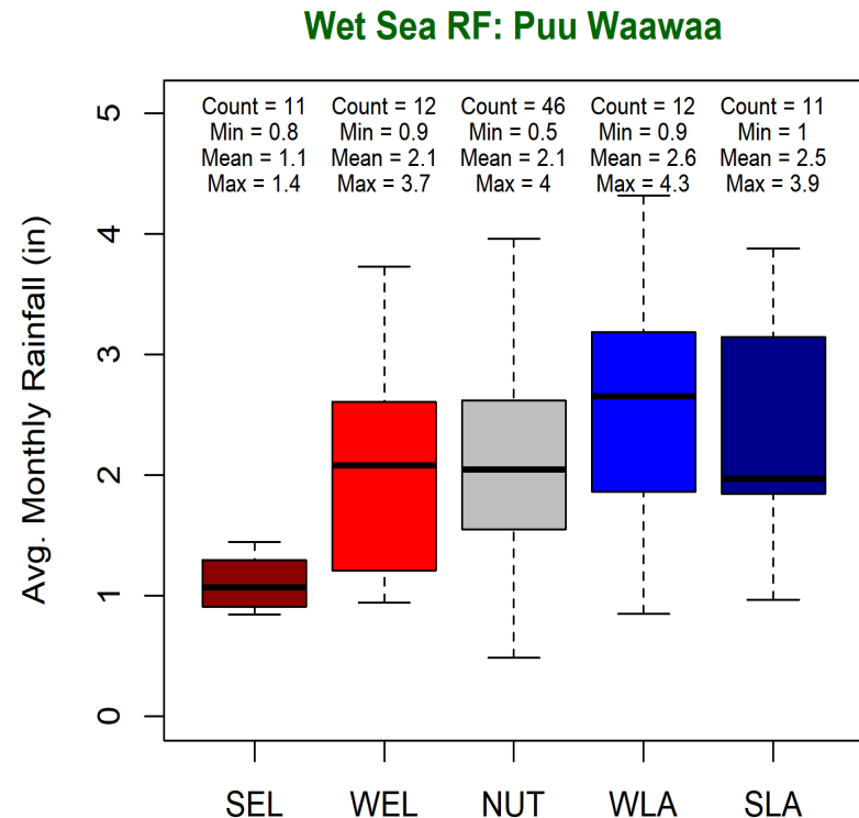
Figure 8. Boxplot of wet season monthly rainfall grouped by ENSO category. Pu'u Wa'awa'a.
