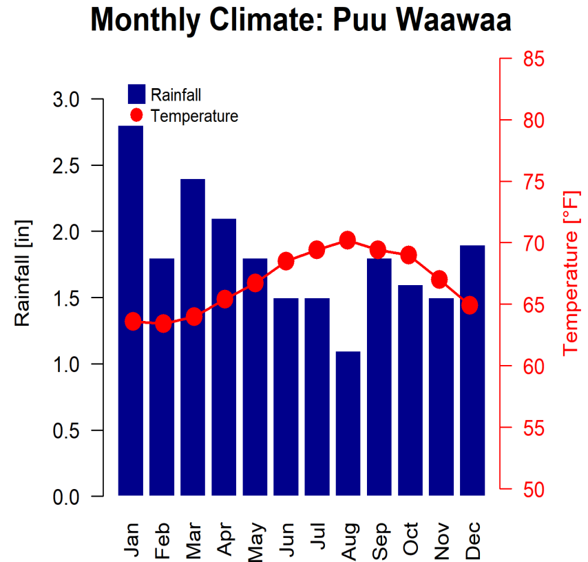
Figure 4. Mean monthly rainfall and temperature at Pu'u Wa'awa'a.
