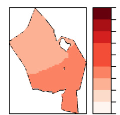
StDs ANN RCP 4.5 (3 °F)
