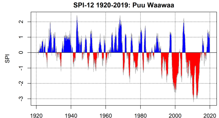
Figure 10. 100-year (1920-2019) SPI-12 time series at Pu'u Wa'awa'a positive SPI (blue) indicate wet periods, negative SPI (red) indicate dry periods.
