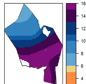
Figure 7. Dry and Wet season total rainfall at Pu'u Wa'awa'a.
