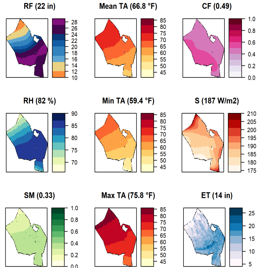
Figure 3. Mean annual climate of Pu'u Wa'awa'a with area average shown in heading of each plot.
