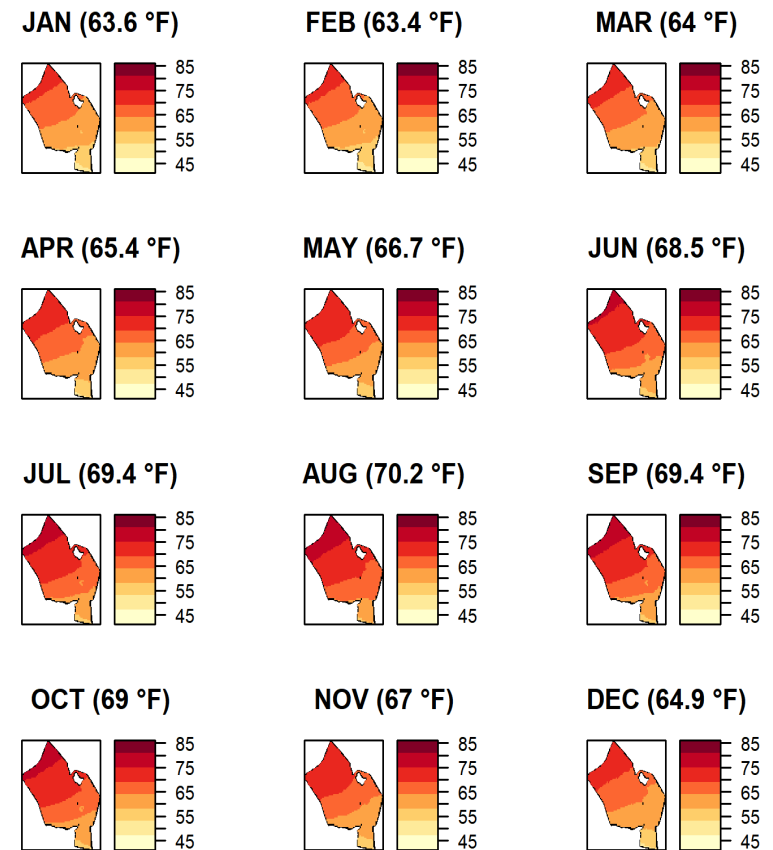
Figure 6. Mean monthly temperature at Pu'u Wa'awa'a with area average shown in heading of each plot.
