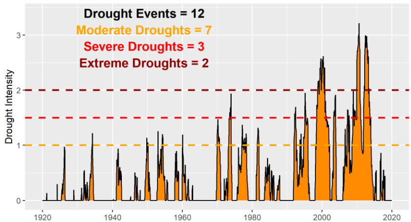
SPI-12 Drought Events 1920 -2019: Puu Waawaa
