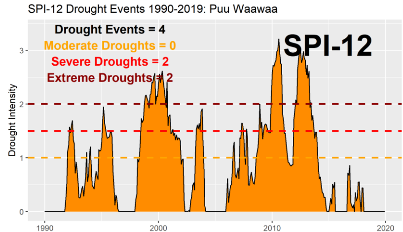
Figure 13. 30-year (1990-2019) SPI-12 time series (reversed axis) at Pu'u Wa'awa'a.
