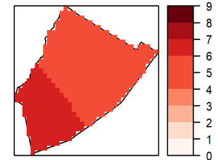
Figure 17. Downscaled projected change in mean temperature (Year 2100) at Laupāhoehoe NAR, Dynamical Downscaling (DyDs), Statistical Downscaling (StDs).
