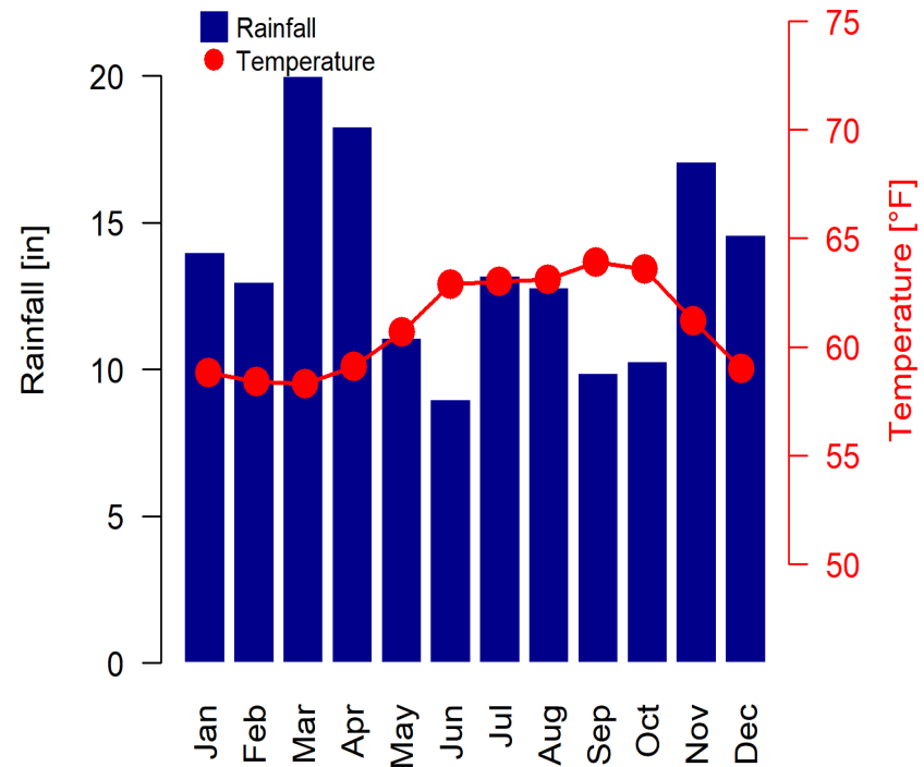
Figure 4. Mean monthly rainfall and temperature at Laupāhoehoe NAR.
