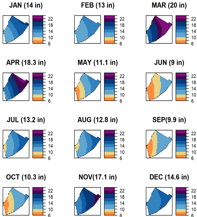
Figure 5. Mean monthly rainfall Laupāhoehoe NAR with area average shown in heading of each plot.
