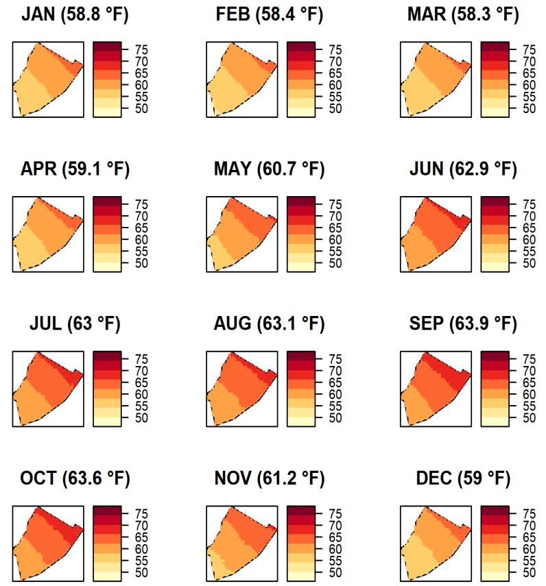
Figure 6. Mean monthly temperature at Laupāhoehoe NAR with area average shown in heading of each plot.
