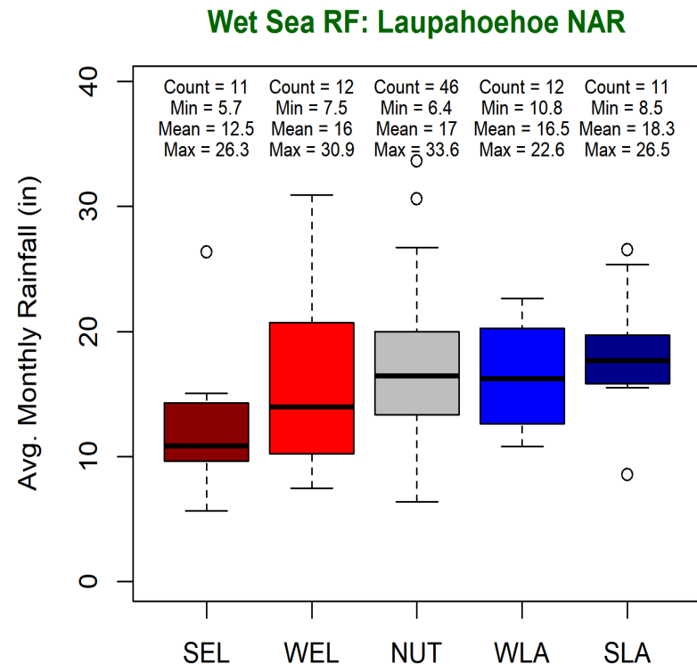
Figure 8. Boxplot of wet season monthly rainfall grouped by ENSO category. Laupāhoehoe NAR.
