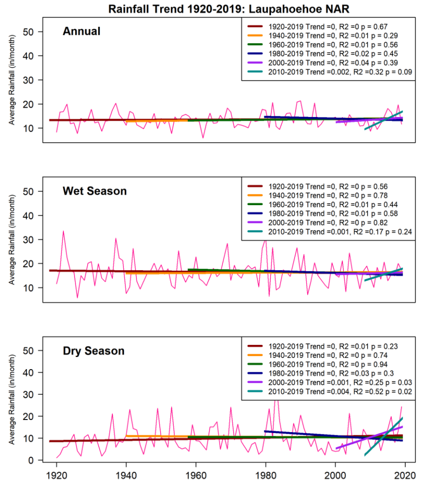
Figure 9. 100-year (1920-2019) rainfall time series at Laupāhoehoe NAR with linear trends calculated over six unique periods in the record; Trend is the slope ( inches per year); R2 is the strength of the trend; p is a measure of the statistical significance.
