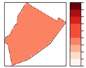
Figure 17. Downscaled projected change in mean temperature (Year 2100) at Laupāhoehoe NAR, Dynamical Downscaling (DyDs), Statistical Downscaling (StDs).
