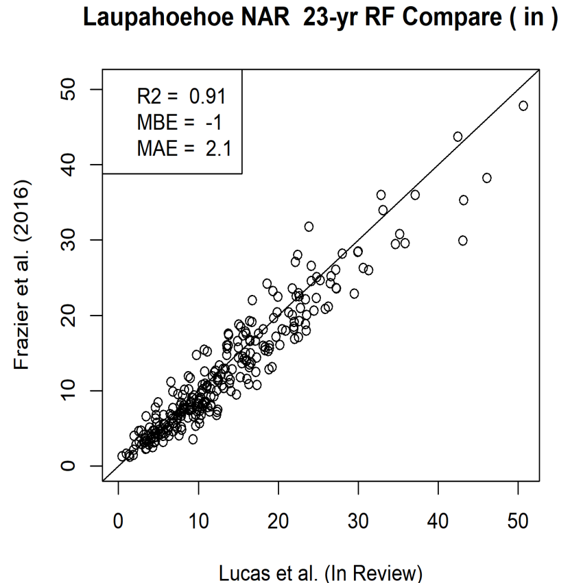
Figure A1: One to one comparison of 23-years (1990-2012) of monthly rainfall from two unique datasets for Laupāhoehoe NAR, and associated error metrics; R2, is the coefficient of determination, MBE, is the mean bias error, MAE, mean absolute error.
