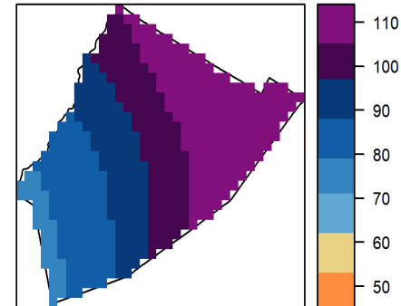
Figure 7. Dry and Wet season total rainfall at Laupāhoehoe NAR.
