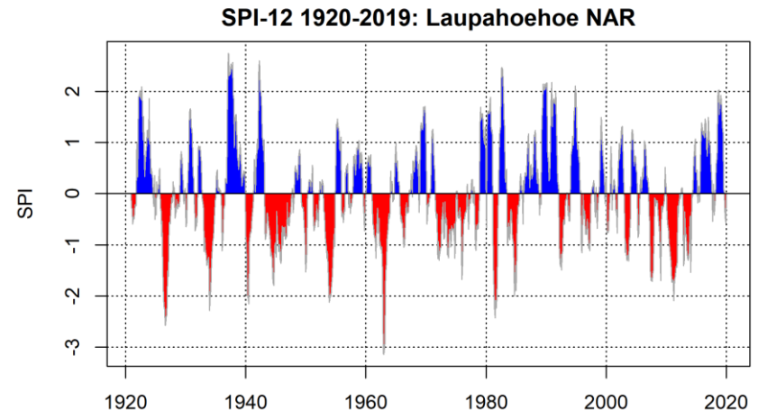
Figure 10. 100-year (1920-2019) SPI-12 time series at Laupāhoehoe NAR positive SPI (blue) indicate wet periods, negative SPI (red) indicate dry periods.
